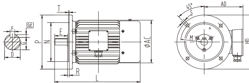
H80~160-IM B5/V1
