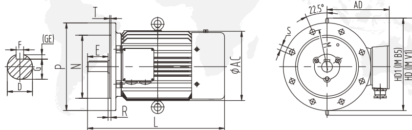
H225~280-IM B5/V1
