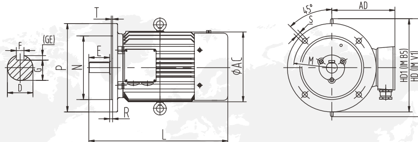
H80~160-IM B5/V1
